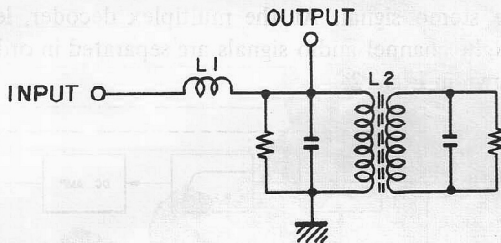
Fig. 5 Double Tuning Type
