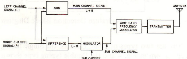
Fig. 10 FM Broadcasting System Diagram
