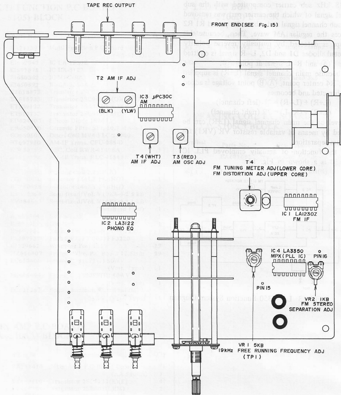
Fig. 14 Multi Function P.C Board AA-5105
