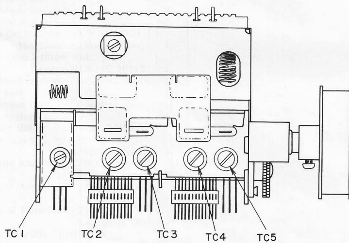
Fig. 15 Front End
