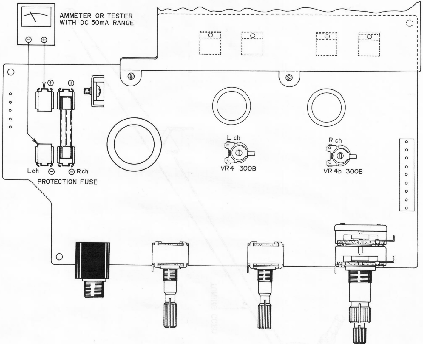
Fig. 17 Main Amp P.C Board AA-5106
