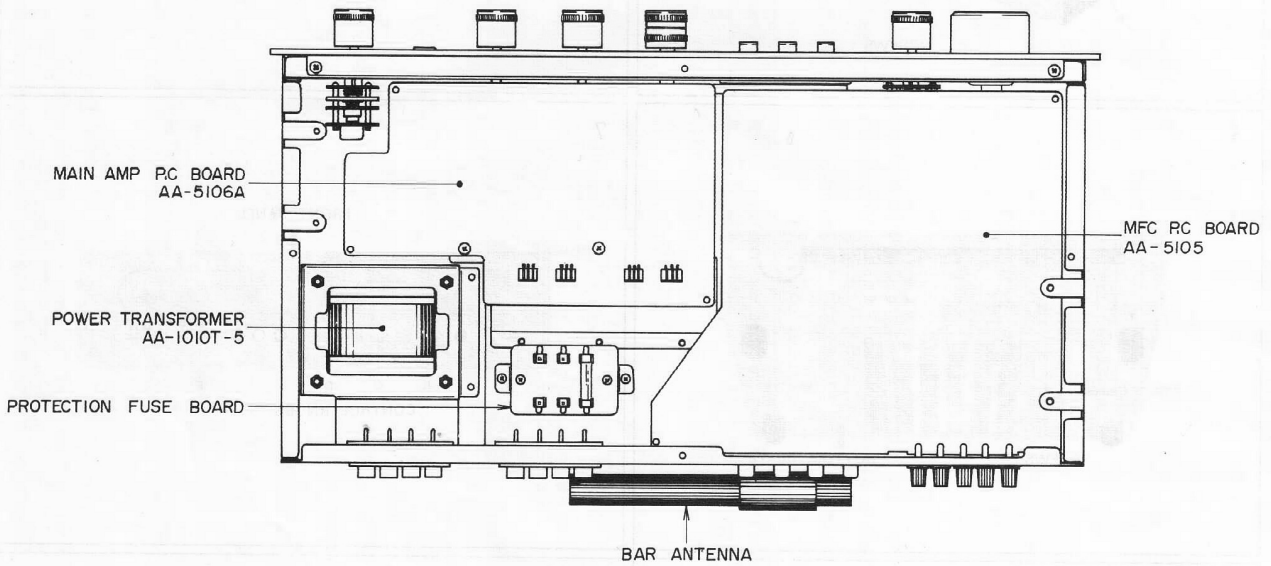
Fig. 2 Bottom View
