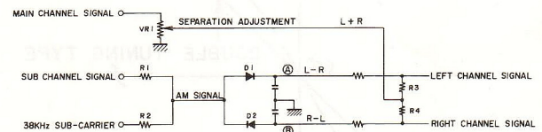
Fig. 12 Multiplex Decoder
