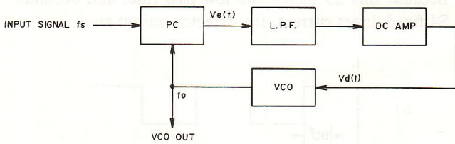
Fig. 9 PLL Circuit
