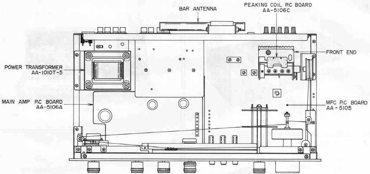
Fig 1 Top View
