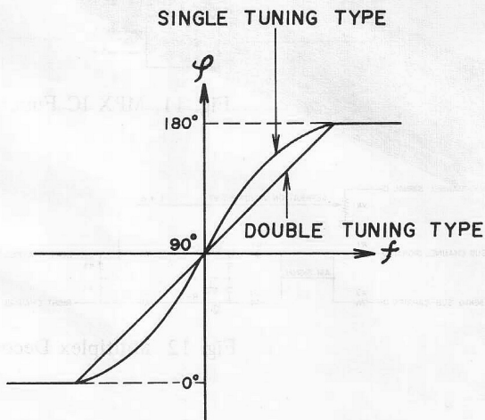
Fig. 6 Tuning Curve
