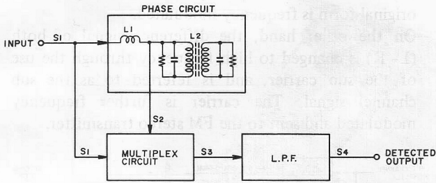
Fig. 3 Quadrature Detection Block Diagram
