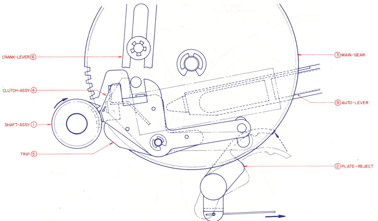
Fig. 13 FORCE CUT
