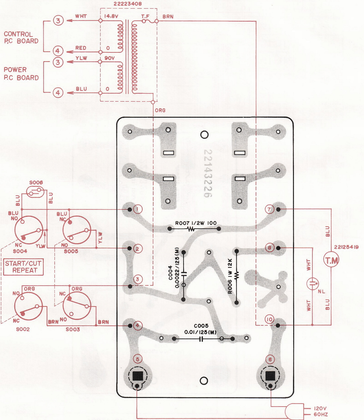
SUPPLY P.C BOARD 22143226 CSA MODEL
