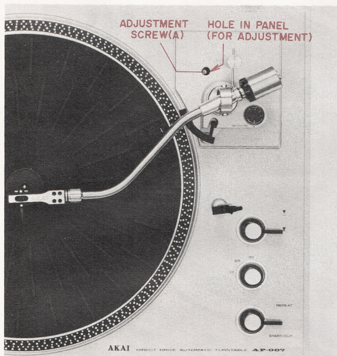
Fig. 11 Lead-in Adjustment
