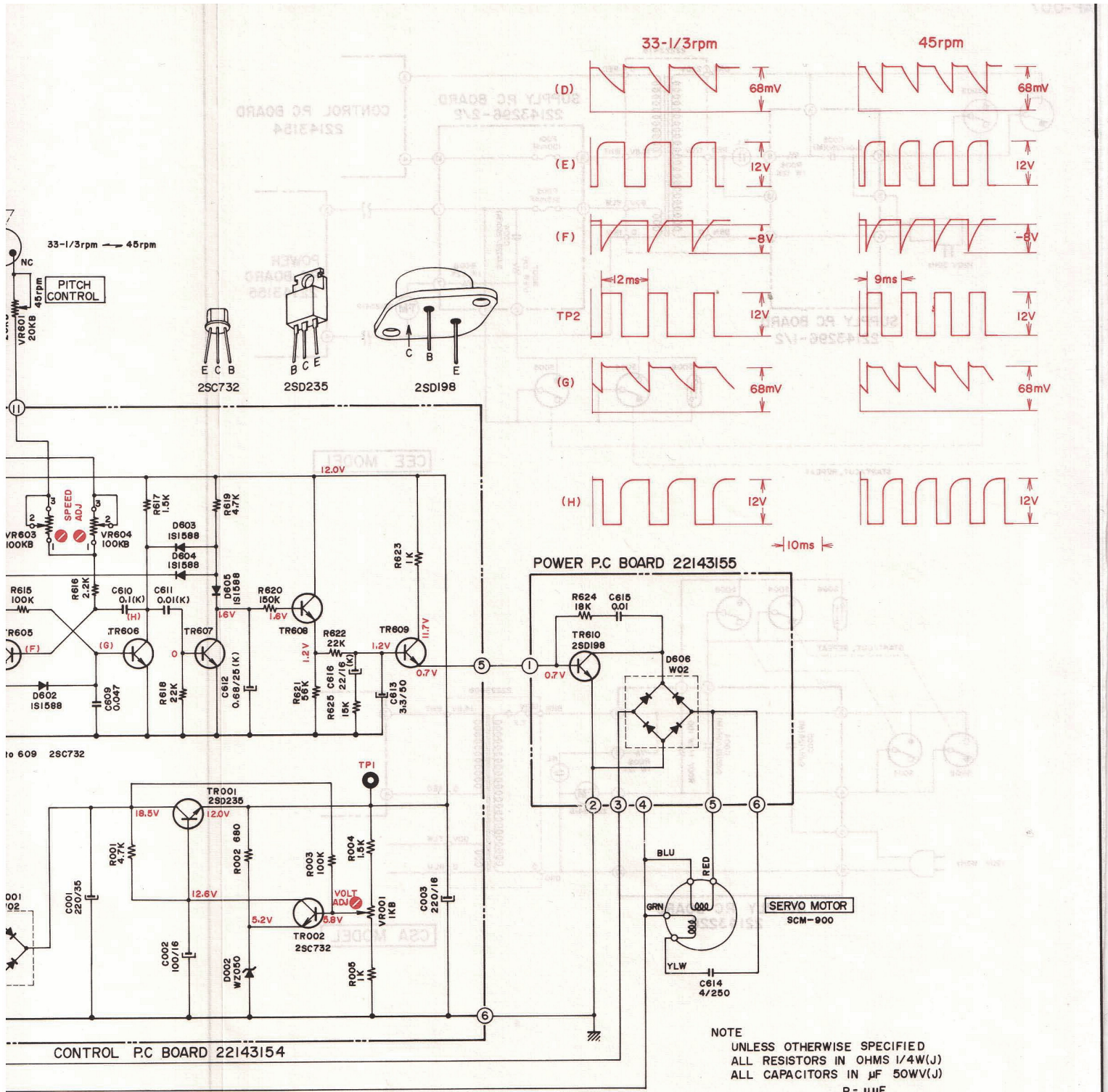
AP-007 SCHEMATIC DIAGRAM NO.2-1 1541402A
