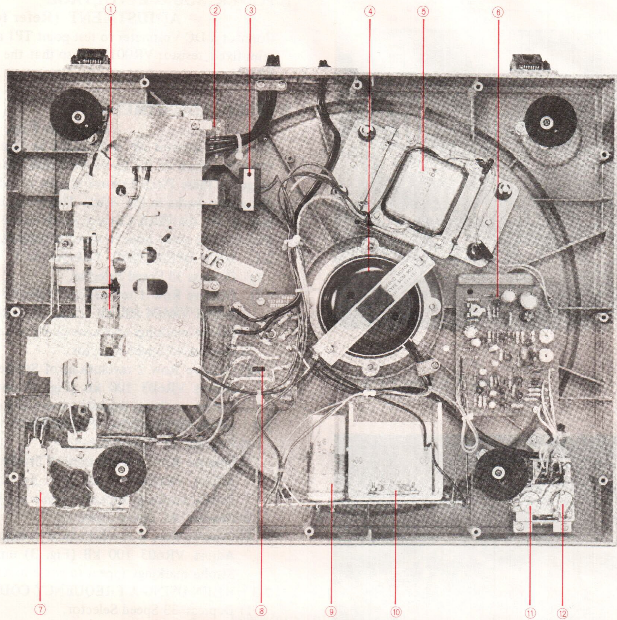
Fig. 2 Bottom View
