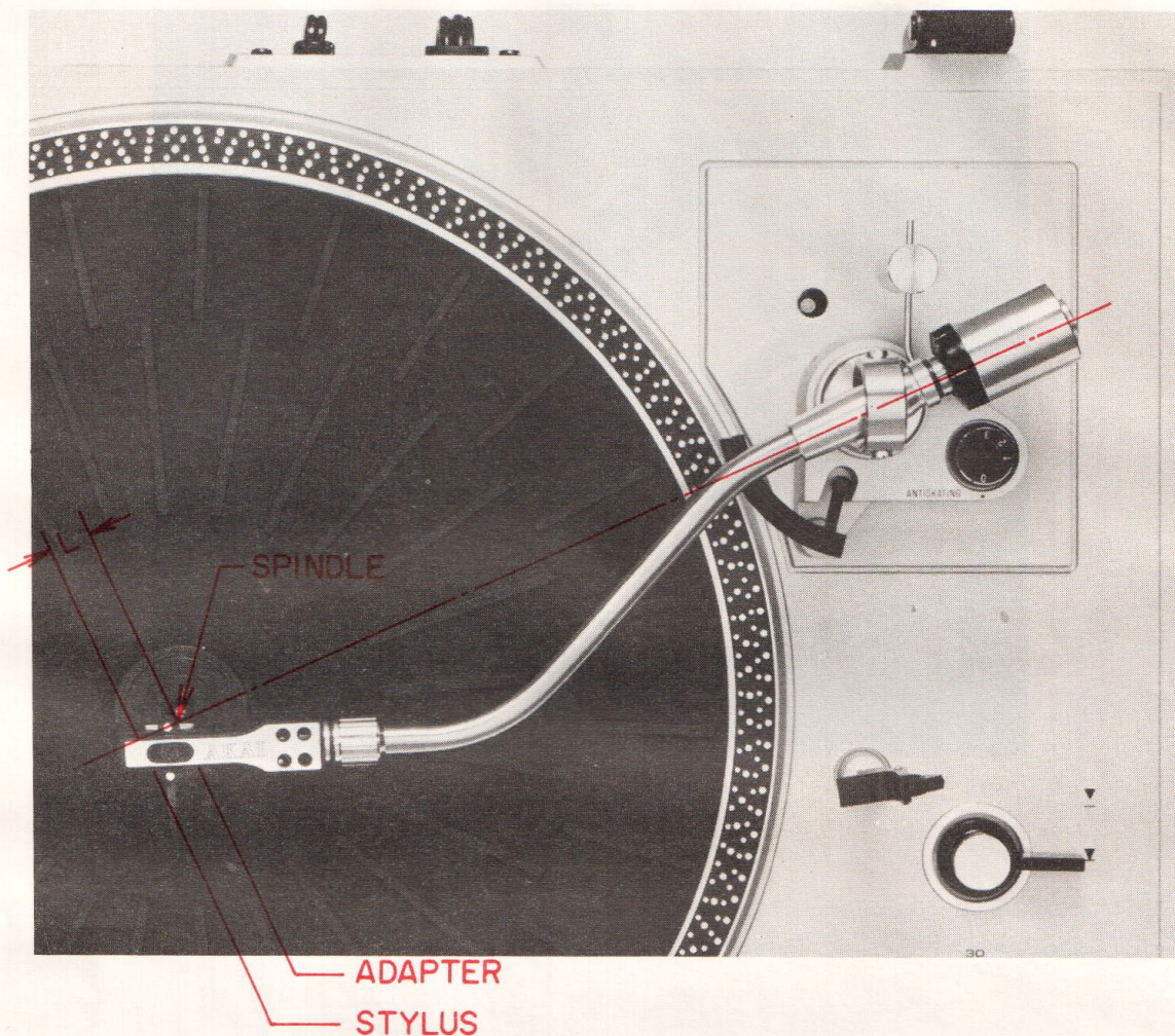
Fig. 7 Overhang Adjustment
