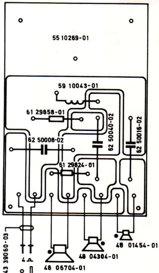
WIRING DIAGRAM
