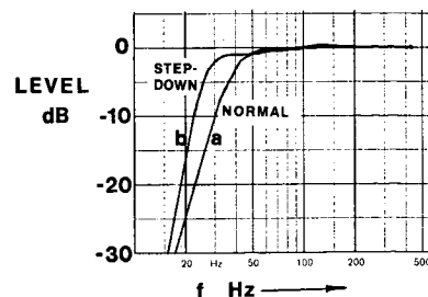
Fig. 2. Display of low-frequency responses for the 380-mm (15-in) driver vented-box system. a —normal unequalized fourth-order Butterworth high-pass configuration with f_3 = f_B = 40 Hz; b —stepped-down equalized sixth-order pseudo-Butterworth configuration with f_3 = f_B = 28 Hz.
