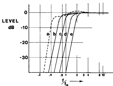
Fig. 1. Selected low-frequency responses from new set of sixth-order assisted vented-box alignments. The frequency axis is normalized to the driver's free-air resonance frequency f_s . a-C_N = 0.25, f_3 = 0.5 f_s ; b-C_N = 0.5, f_3 = 0.707 f_s ; c-C_N = 1, f_3 = f_s (Thiele's alignment 15); d-C_N = 2, f_3 = 1.414 f_s ; e-C_N = 4, f_3 = 2 f_s .
