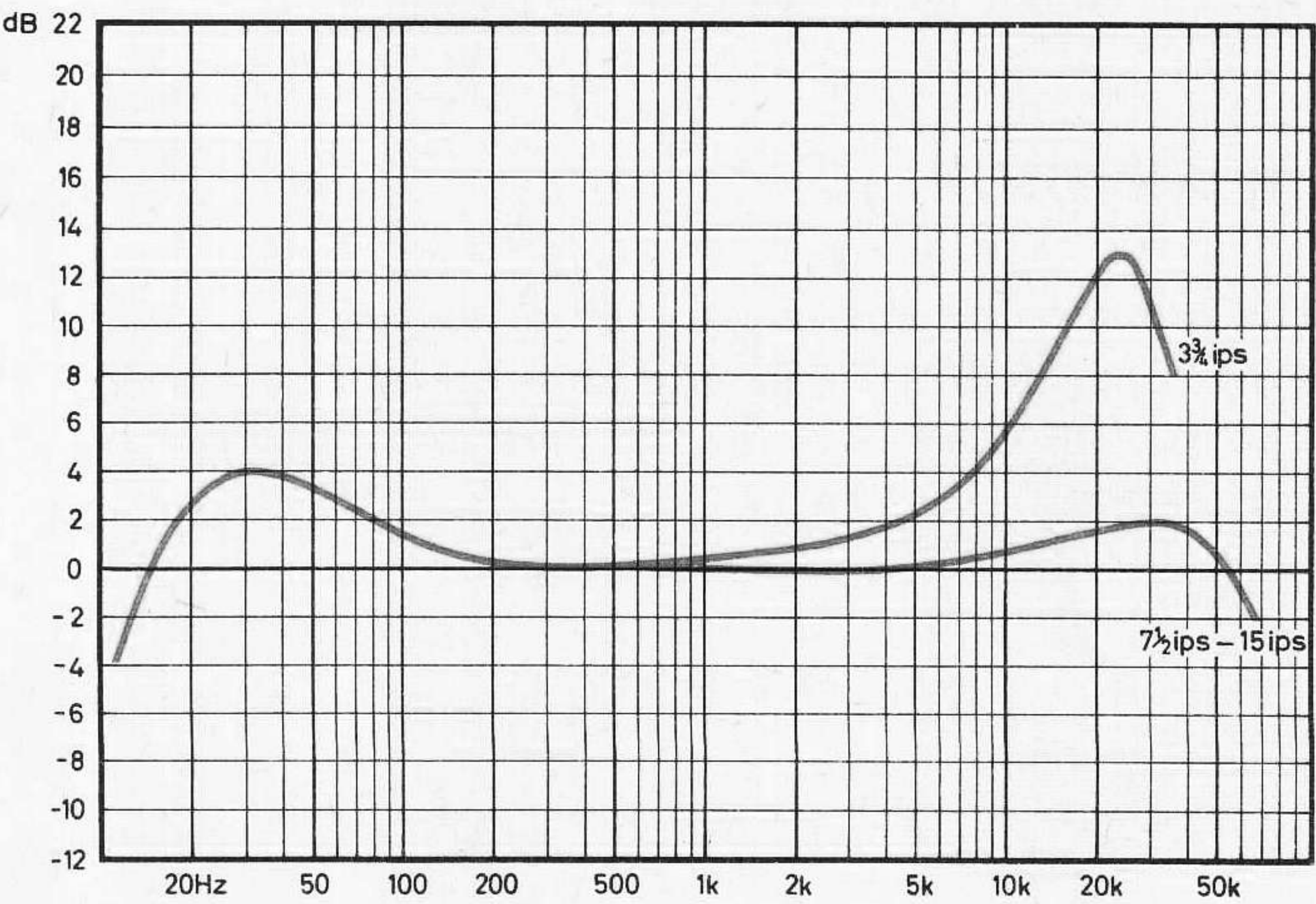
IEC record curve
