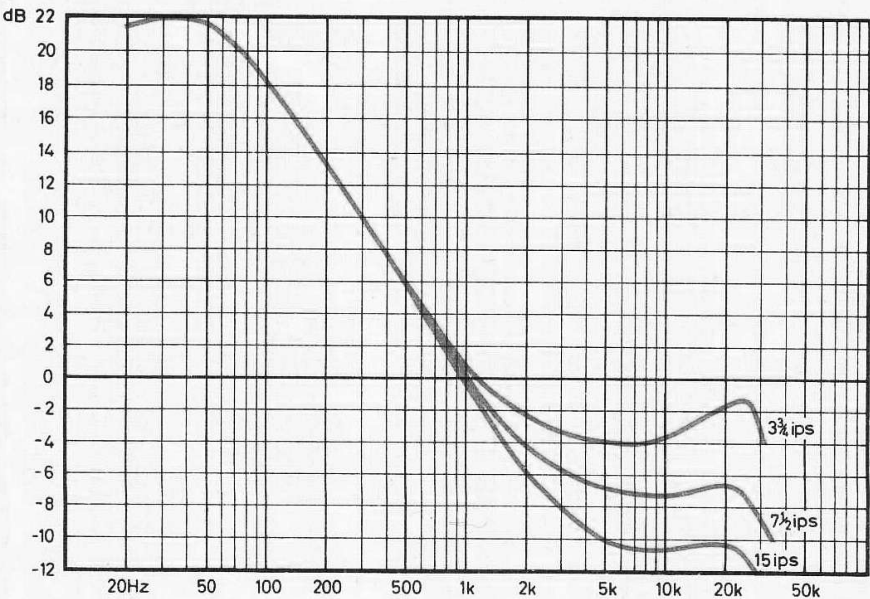
IEC playback curve
