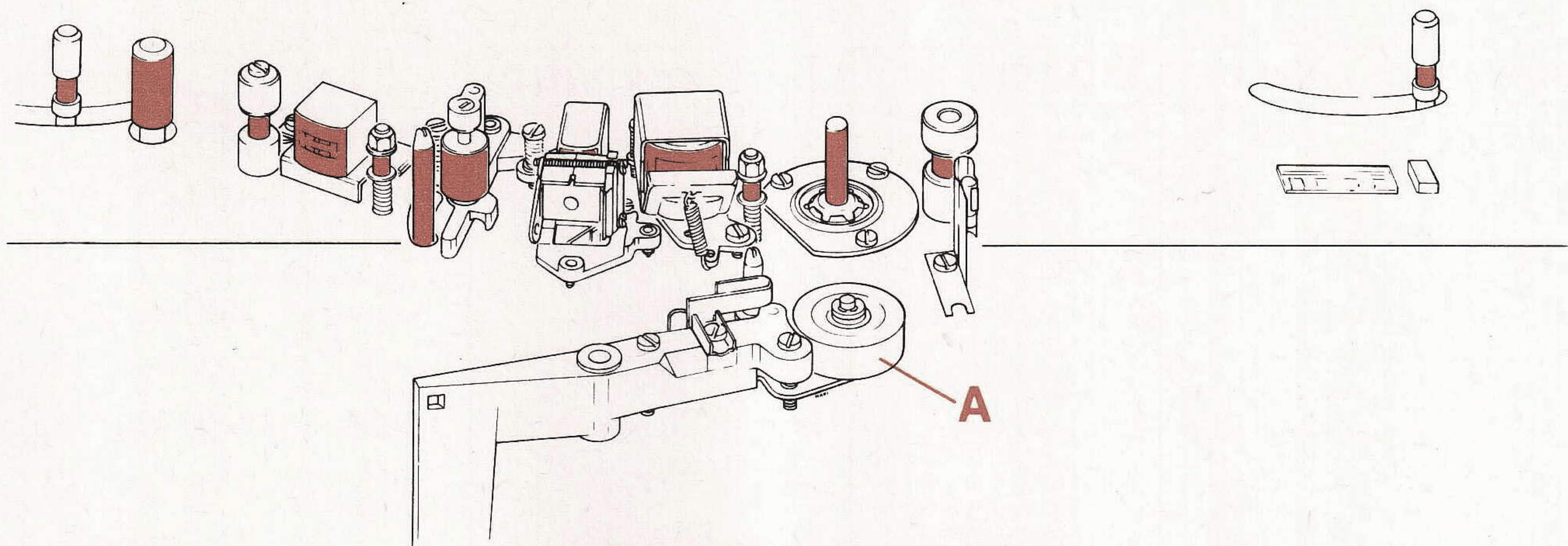
Fig. 2.1 Cleaning the tape path
