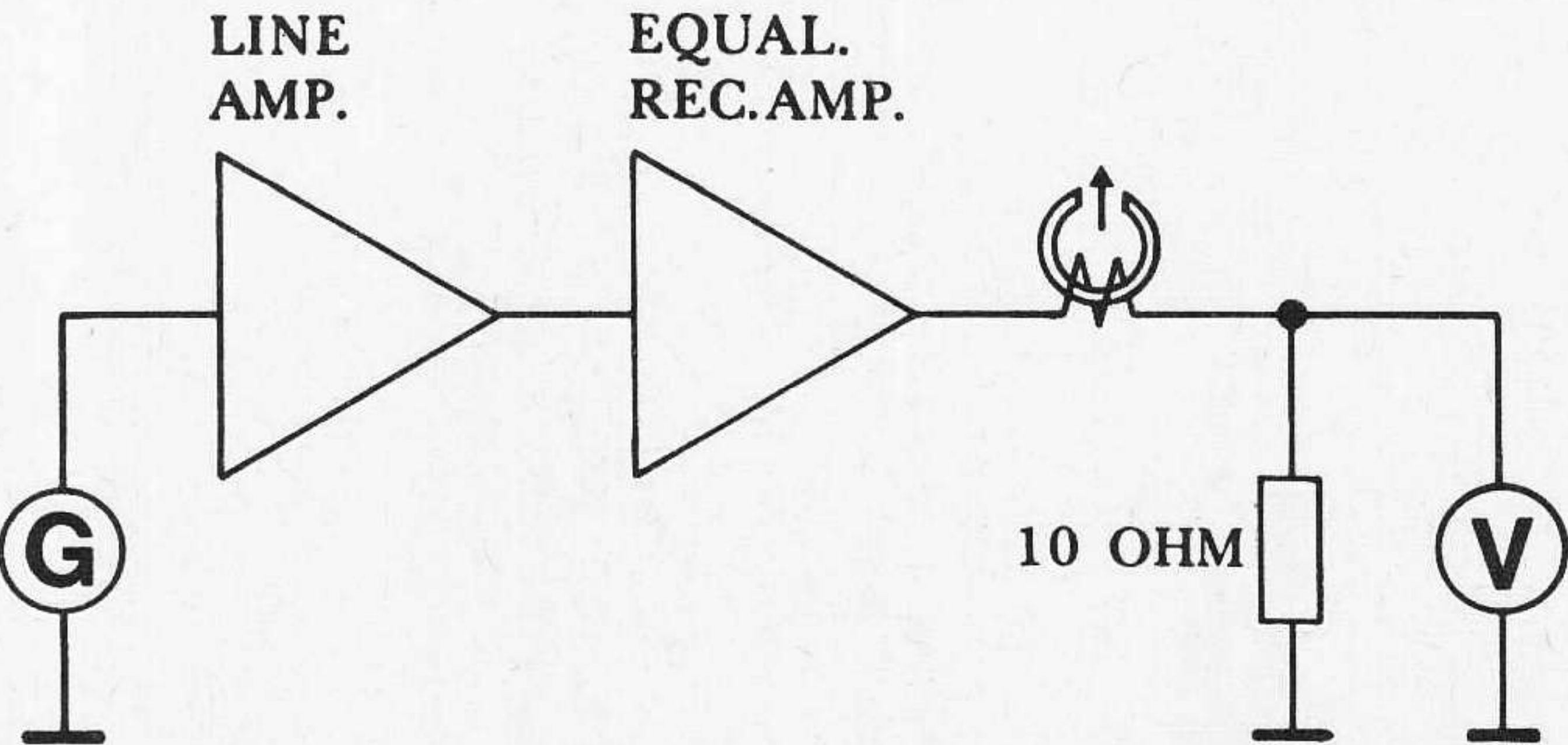
Checking the record curve
