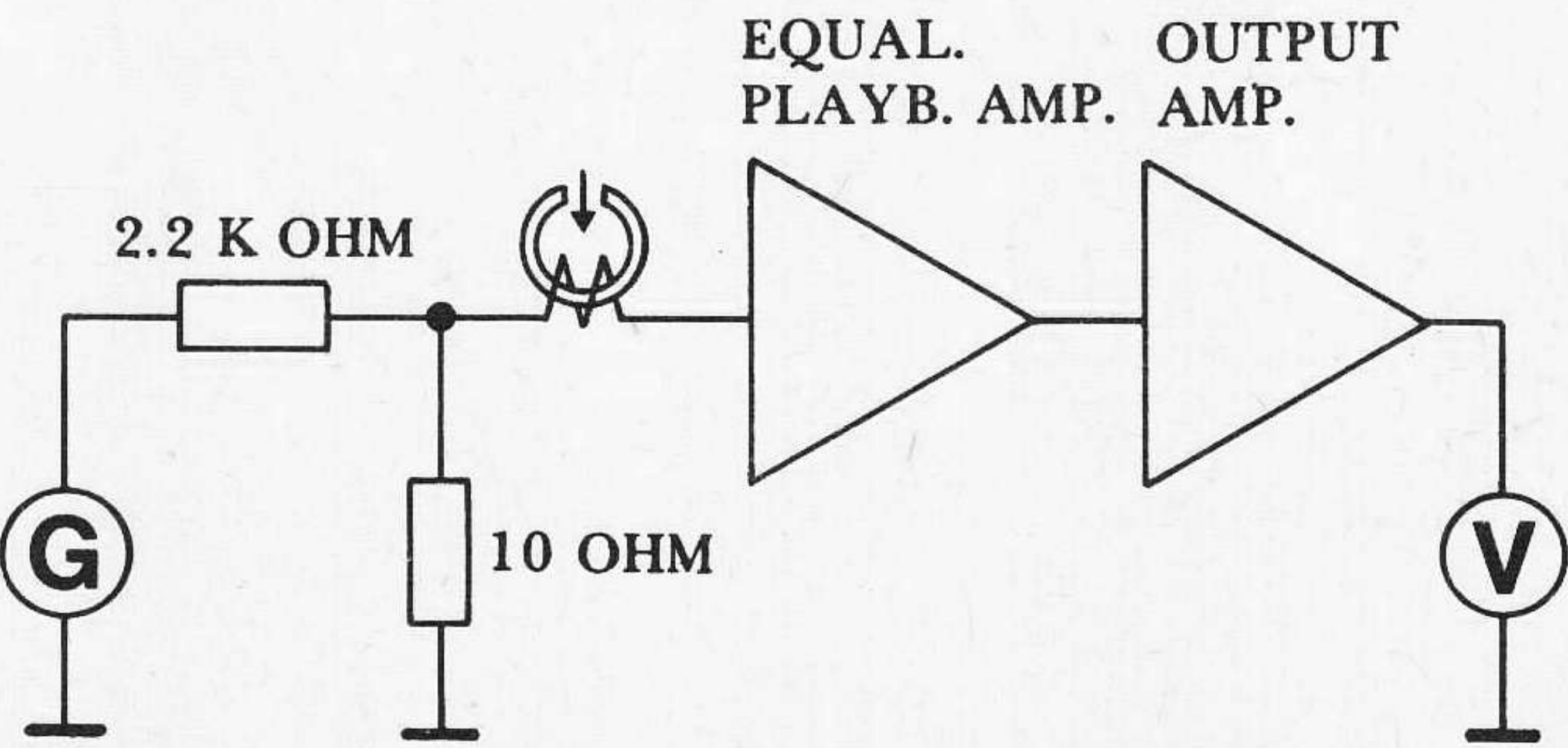
Checking the playback curve
